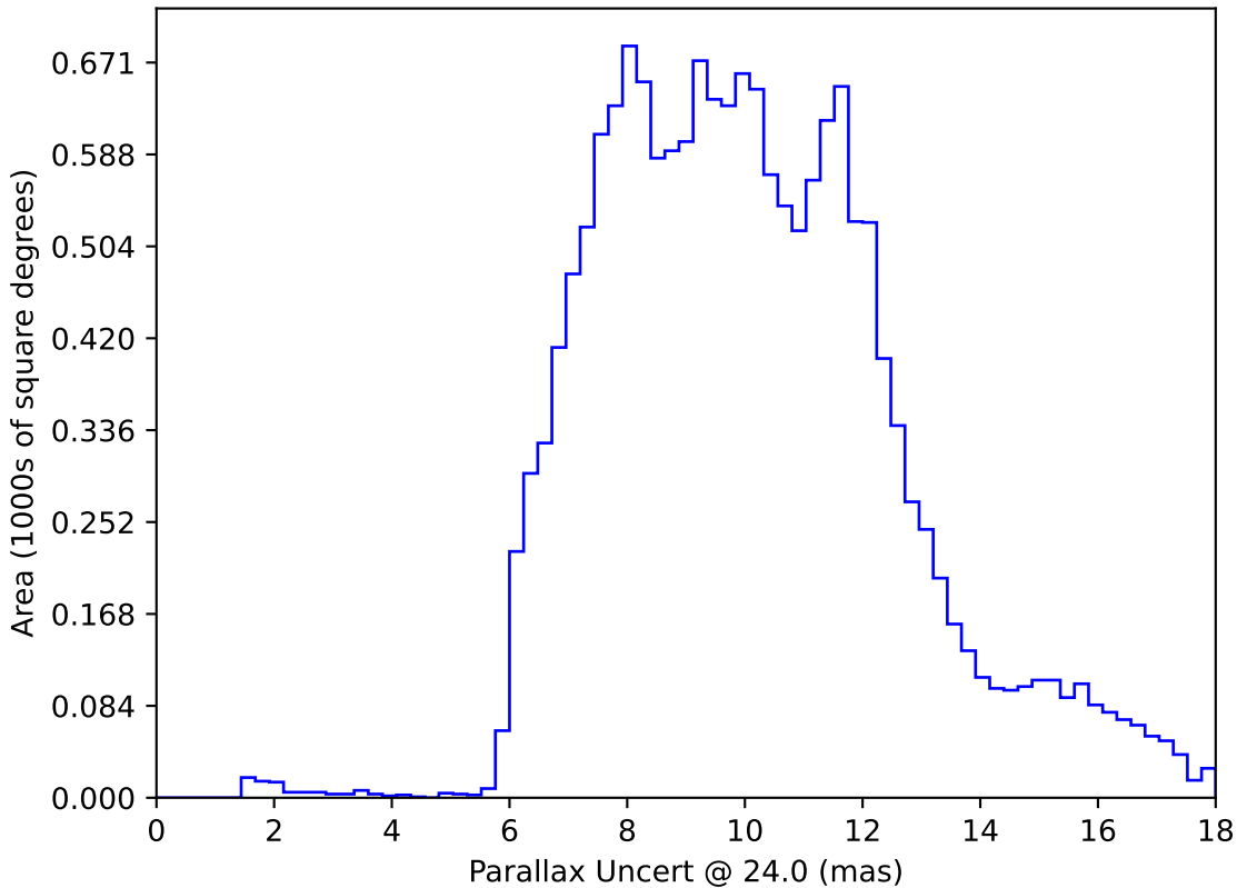
baseline_v3.0_10yrs WFD: Parallax Uncert @ 24.0
