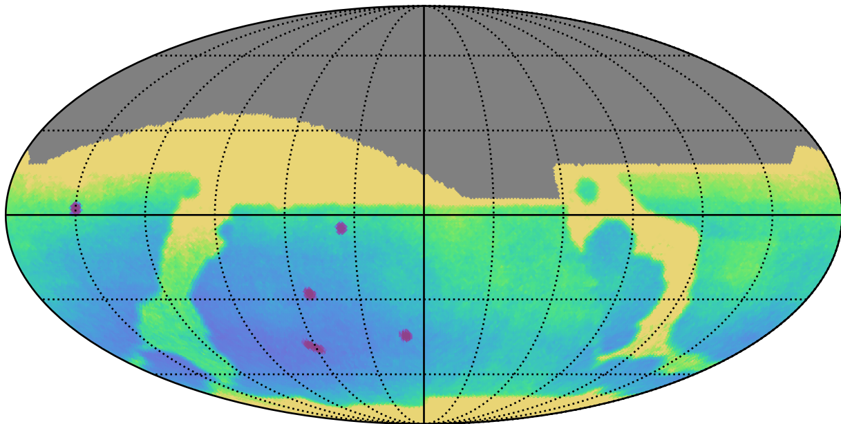
baseline_v3.0_10yrs All sky: Parallax Uncert @ 24.0
