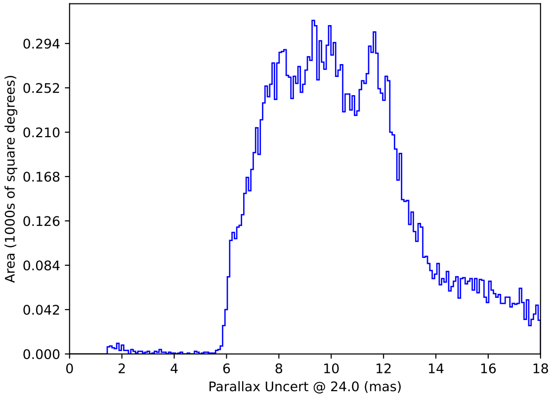
baseline_v3.0_10yrs All sky: Parallax Uncert @ 24.0
