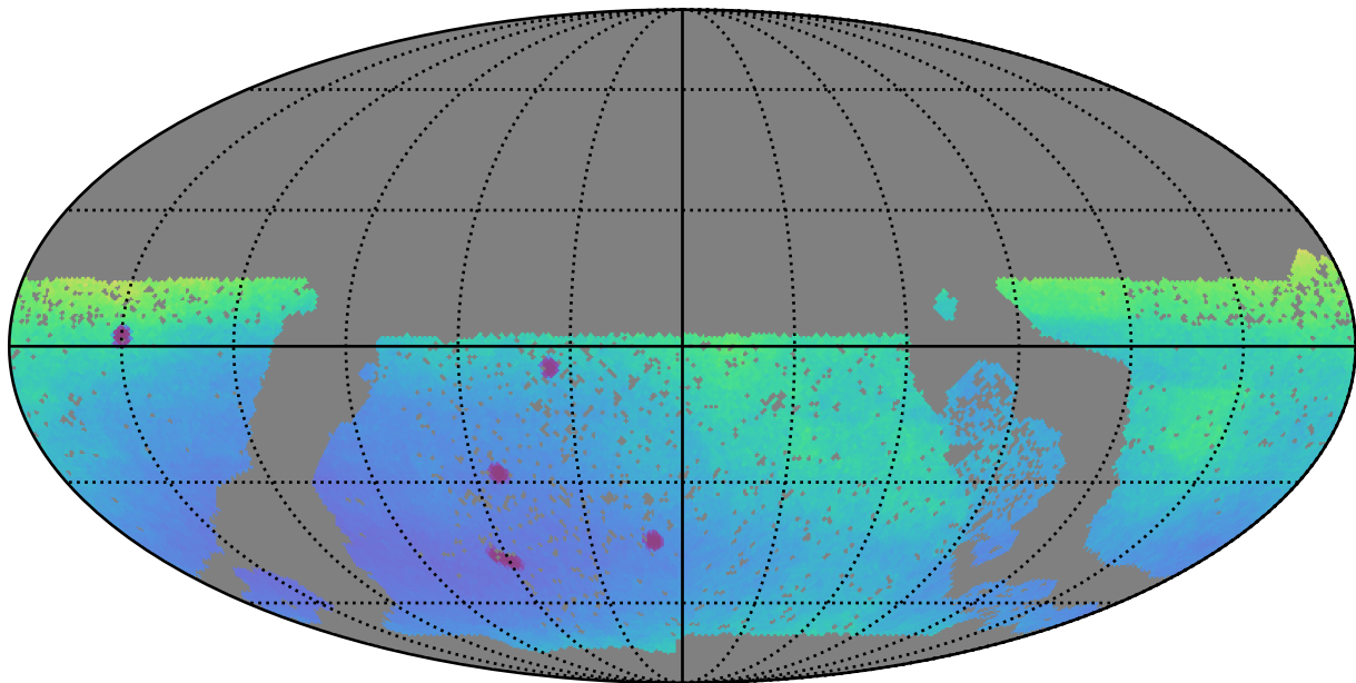
baseline_v3.0_10yrs WFD: Parallax Uncert @ 22.4
