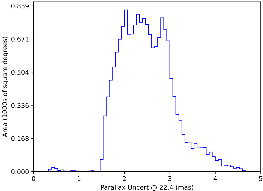
baseline_v3.0_10yrs WFD: Parallax Uncert @ 22.4
