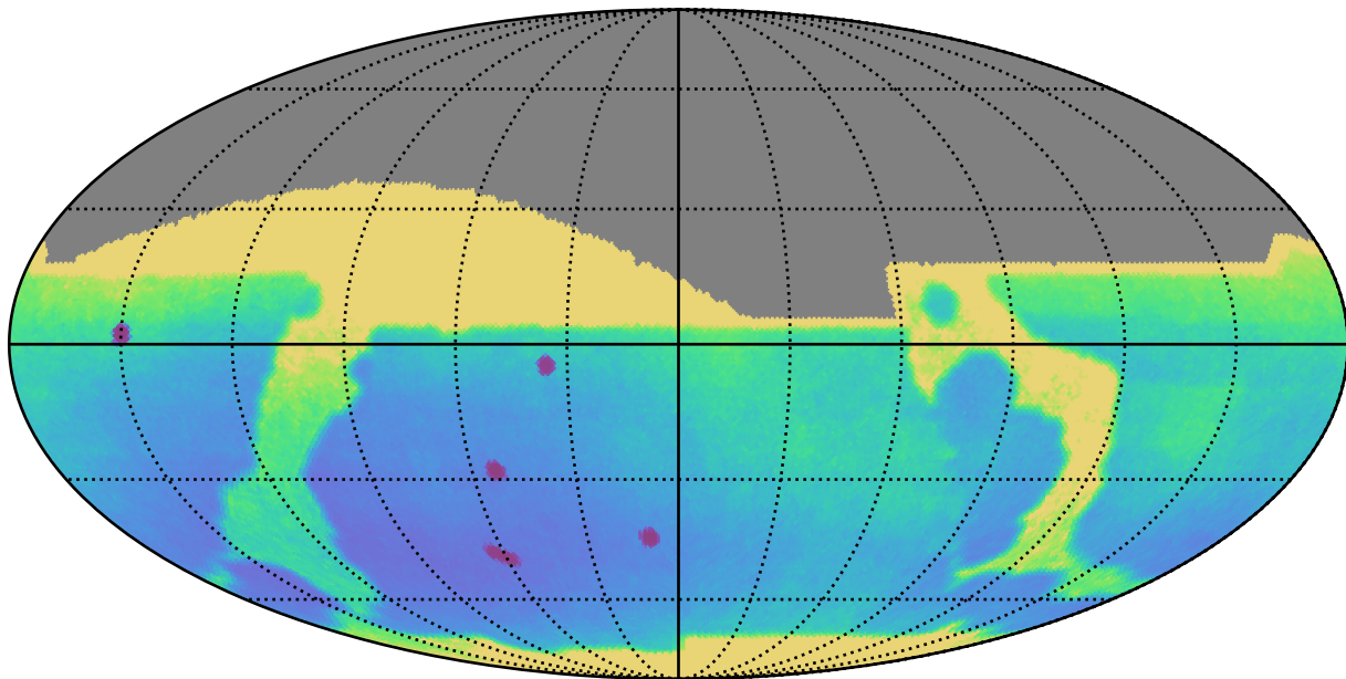
baseline_v3.0_10yrs All sky: Parallax Uncert @ 22.4
