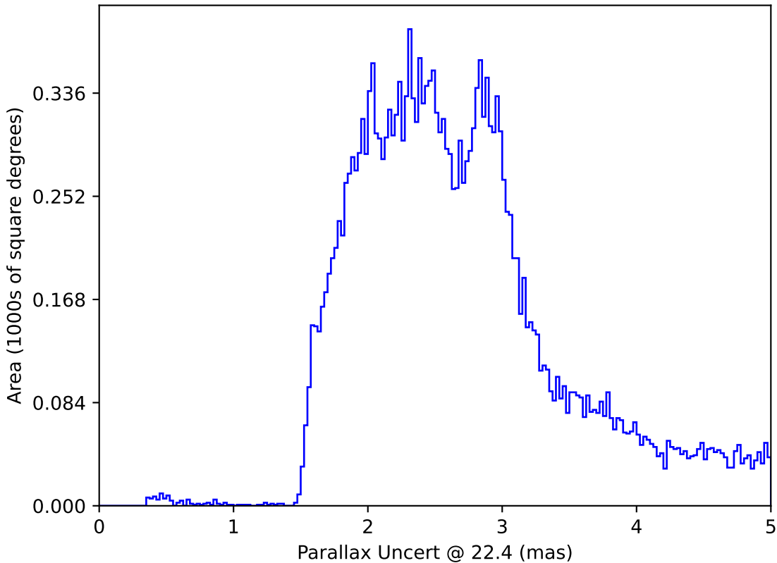
baseline_v3.0_10yrs All sky: Parallax Uncert @ 22.4
