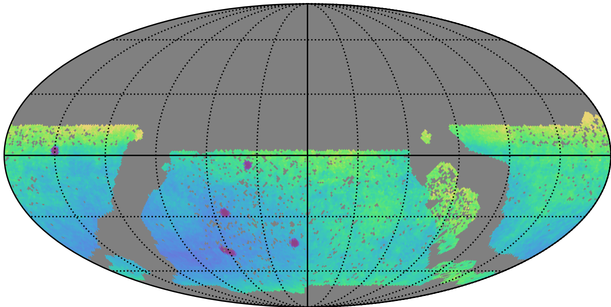
baseline_v3.0_10yrs WFD y band only: Parallax Uncert @ 21.3
