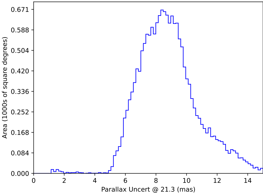
baseline_v3.0_10yrs WFD y band only: Parallax Uncert @ 21.3
