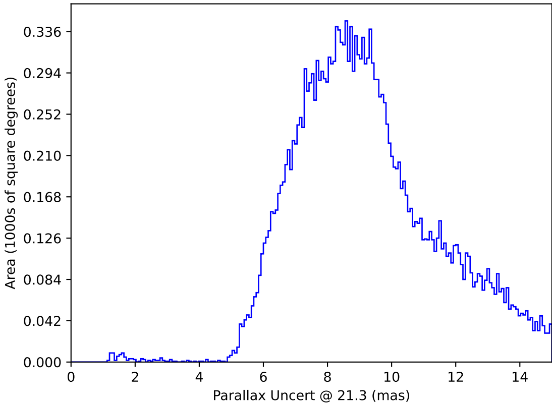
baseline_v3.0_10yrs All sky y band only: Parallax Uncert @ 21.3
