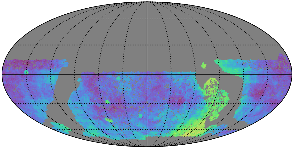
baseline_v3.0_10yrs WFD: Parallax Coverage @ 24.0
