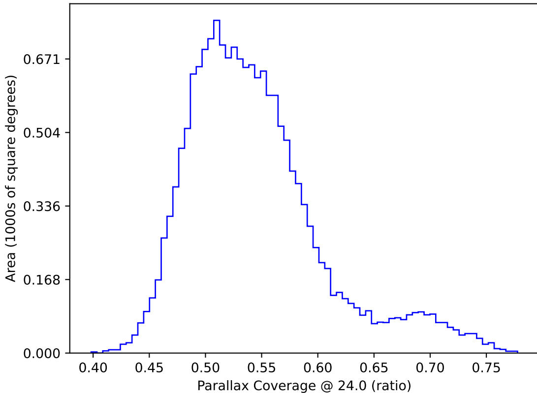
baseline_v3.0_10yrs WFD: Parallax Coverage @ 24.0
