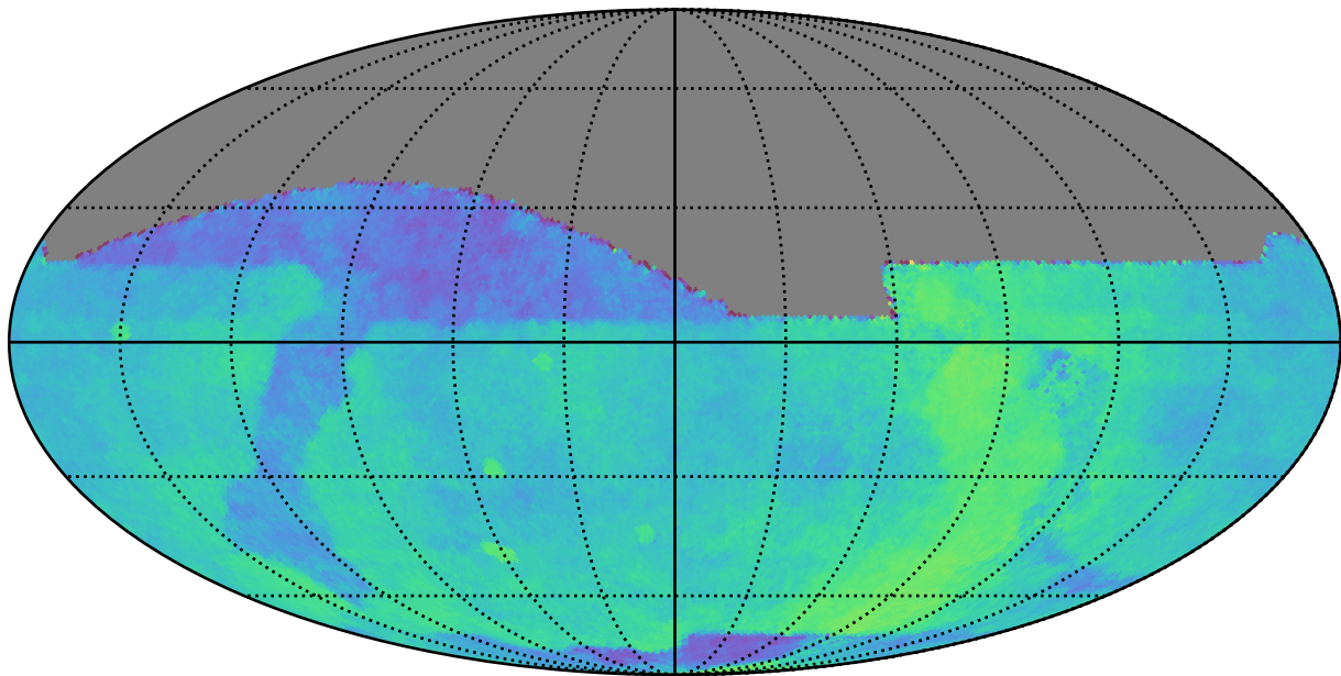
baseline_v3.0_10yrs All sky: Parallax Coverage @ 24.0
