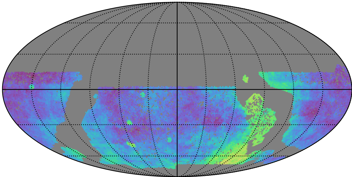
baseline_v3.0_10yrs WFD: Parallax Coverage @ 22.4
