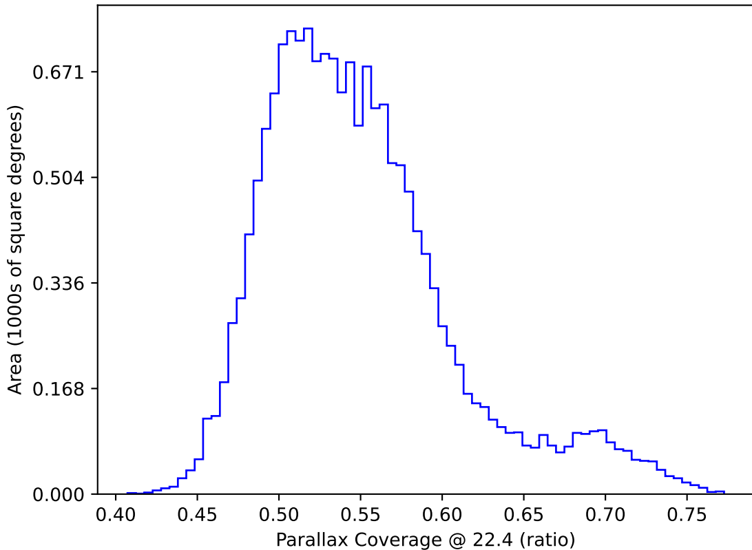
baseline_v3.0_10yrs WFD: Parallax Coverage @ 22.4
