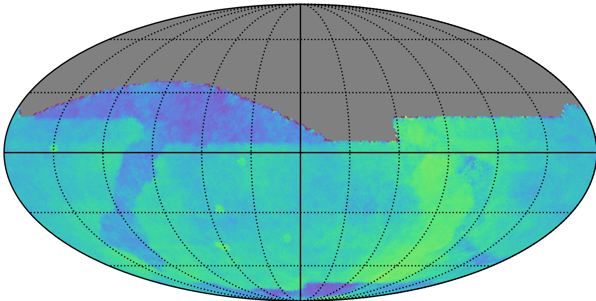
baseline_v3.0_10yrs All sky: Parallax Coverage @ 22.4
