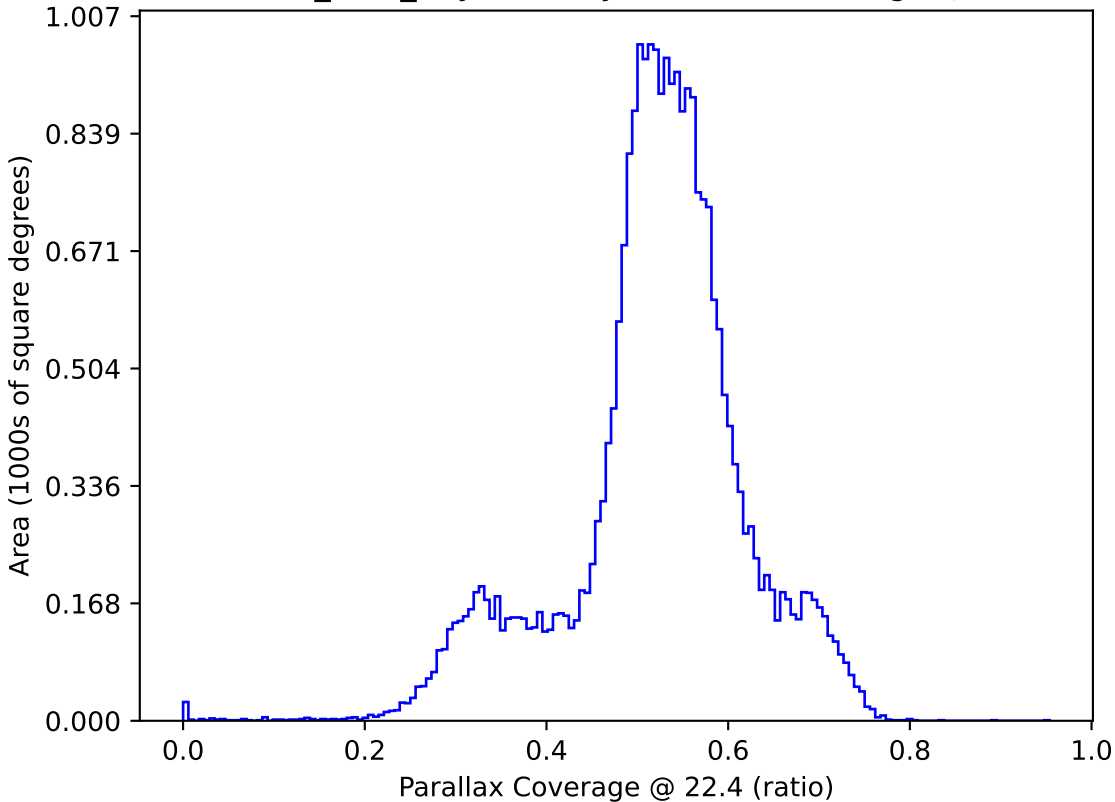
baseline_v3.0_10yrs All sky: Parallax Coverage @ 22.4
