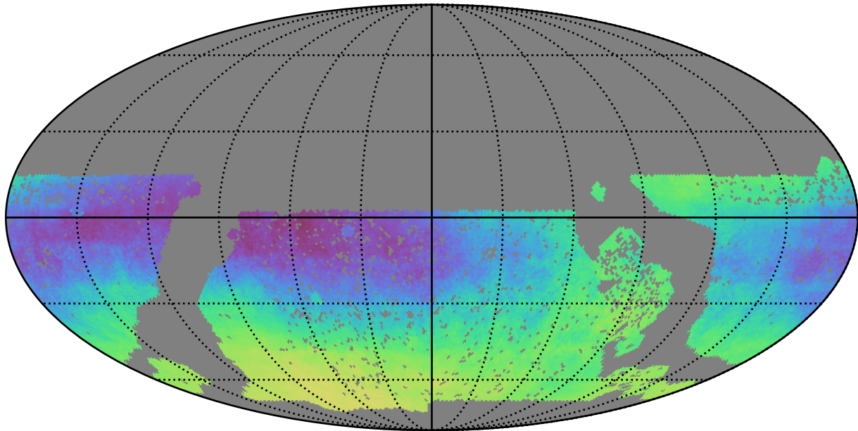
baseline_v3.0_10yrs WFD: Parallax-DCR degeneracy @ 24.0
