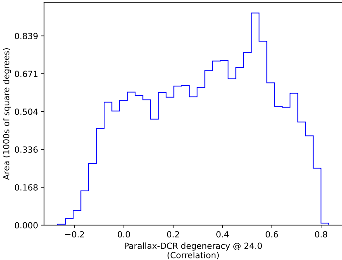
baseline_v3.0_10yrs WFD: Parallax-DCR degeneracy @ 24.0
