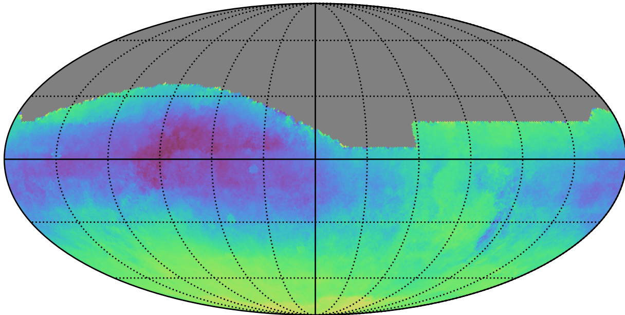
baseline_v3.0_10yrs All sky: Parallax-DCR degeneracy @ 24.0
