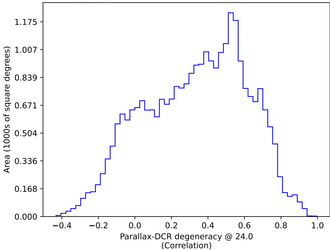
baseline_v3.0_10yrs All sky: Parallax-DCR degeneracy @ 24.0
