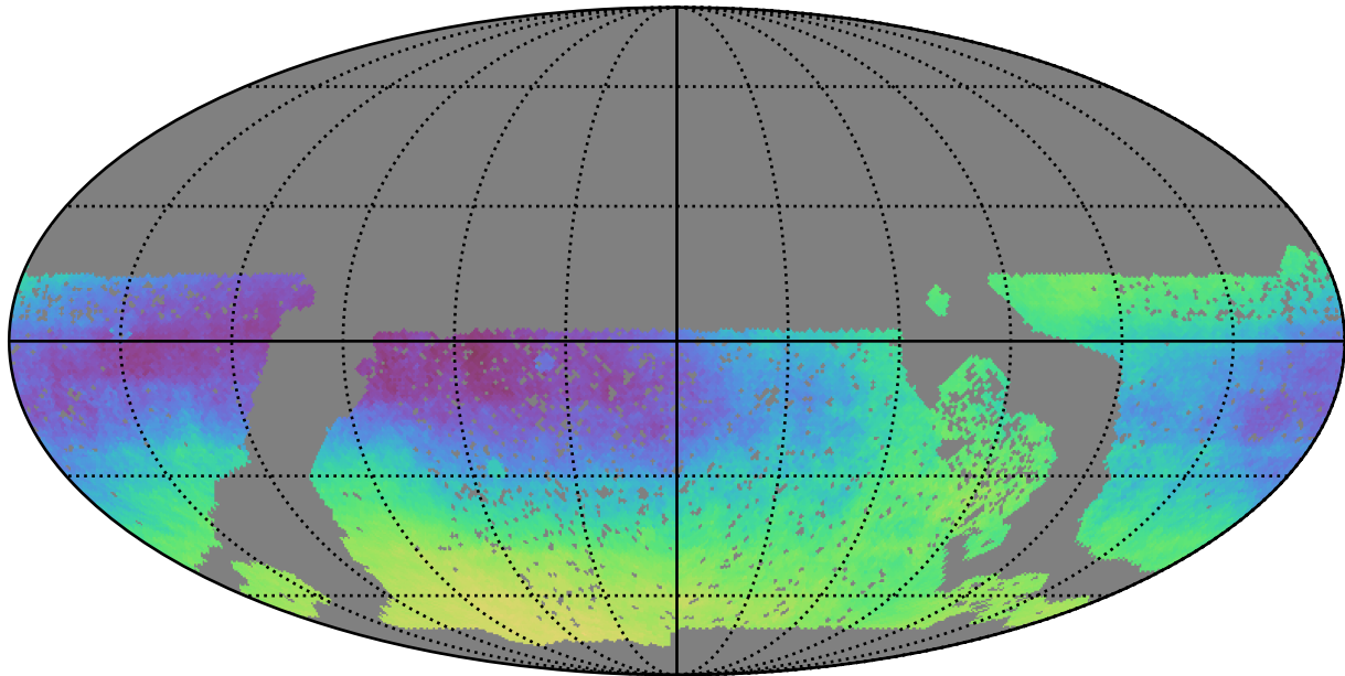
baseline_v3.0_10yrs WFD: Parallax-DCR degeneracy @ 22.4
