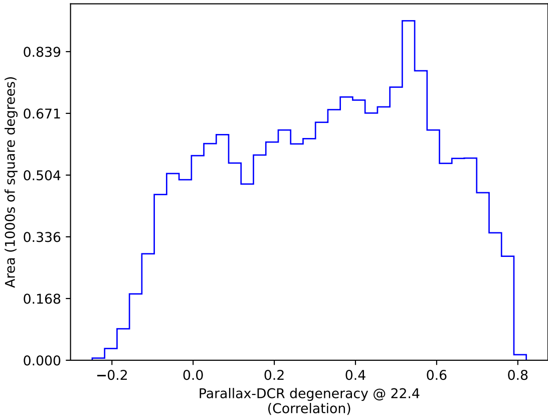
baseline_v3.0_10yrs WFD: Parallax-DCR degeneracy @ 22.4
