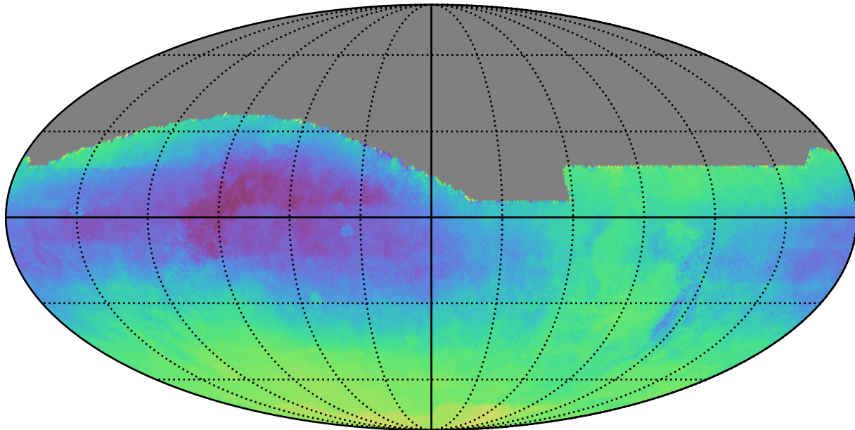
baseline_v3.0_10yrs All sky: Parallax-DCR degeneracy @ 22.4
