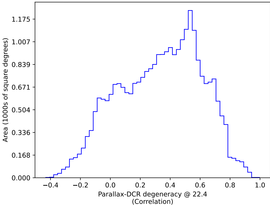
baseline_v3.0_10yrs All sky: Parallax-DCR degeneracy @ 22.4
