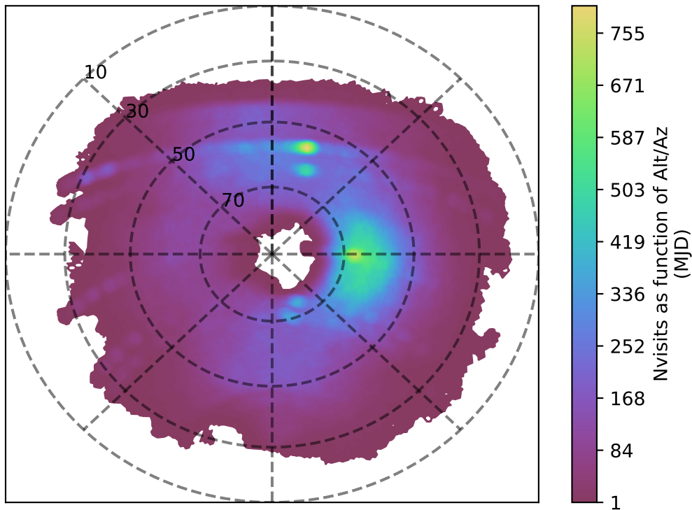
baseline_v3.0_10yrs u band: Nvisits as function of Alt/Az
