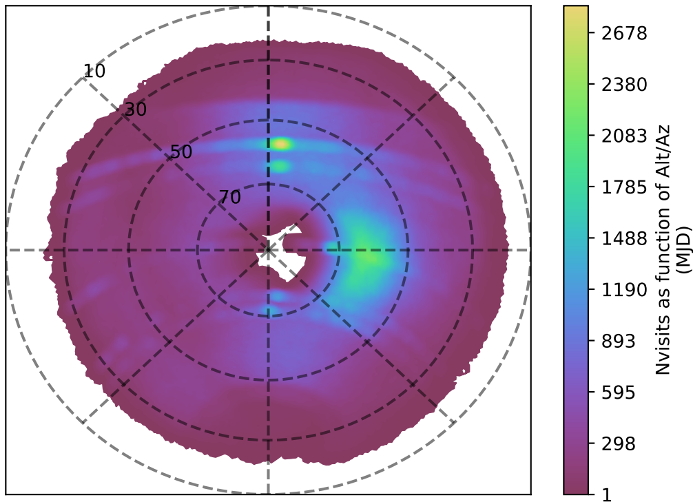
baseline_v3.0_10yrs i band: Nvisits as function of Alt/Az
