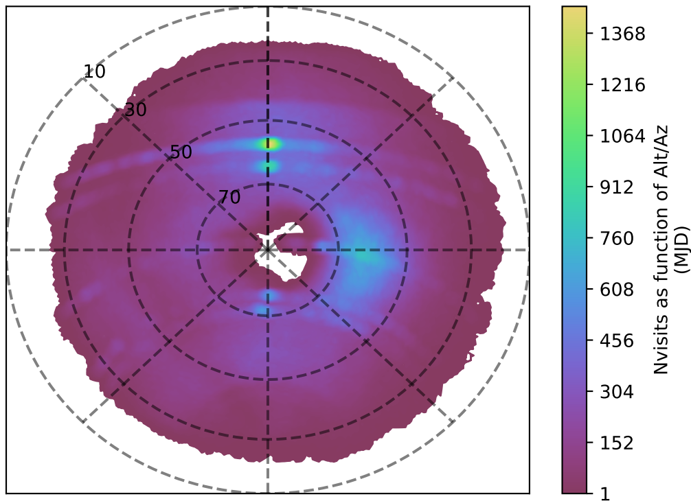
baseline_v3.0_10yrs g band: Nvisits as function of Alt/Az
