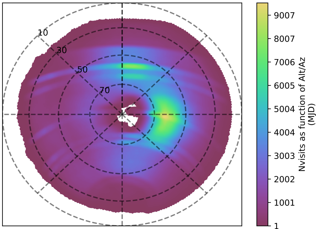
baseline_v3.0_10yrs all bands: Nvisits as function of Alt/Az
