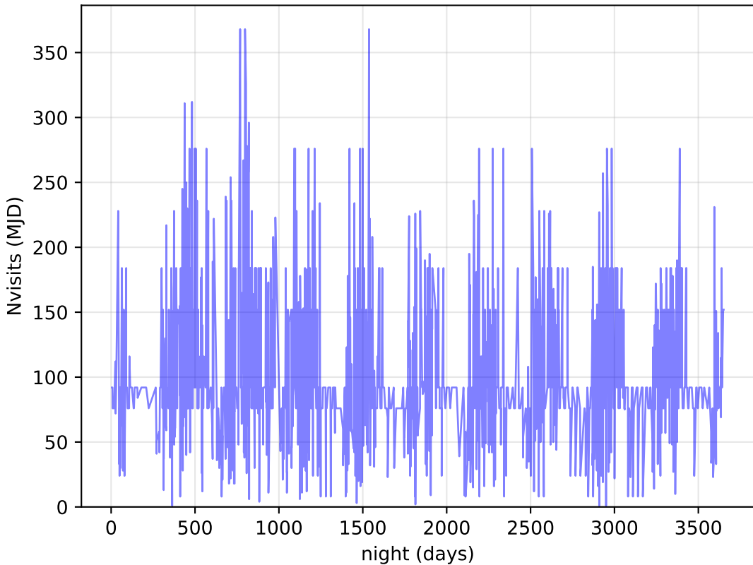
baseline_v3.0_10yrs DDF: Nvisits
