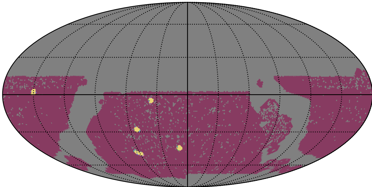
baseline_v3.0_10yrs WFD: NumberOfQuickRevisits
