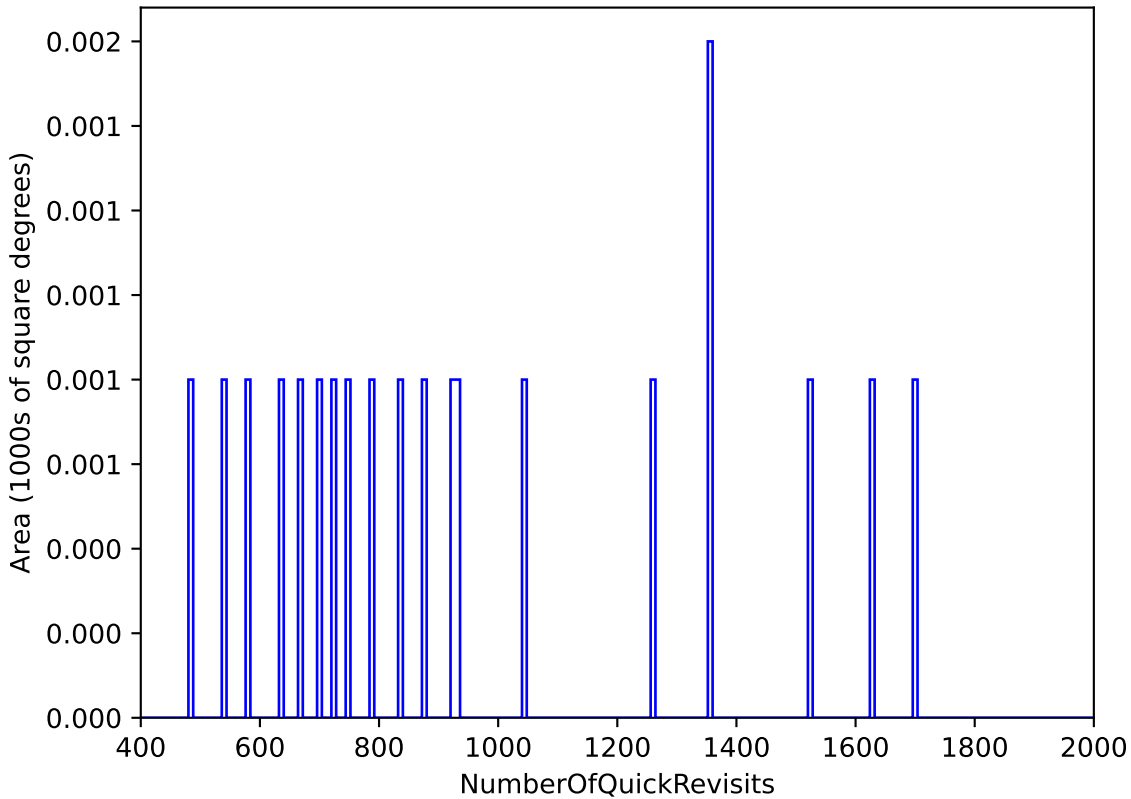
baseline_v3.0_10yrs WFD: NumberOfQuickRevisits
