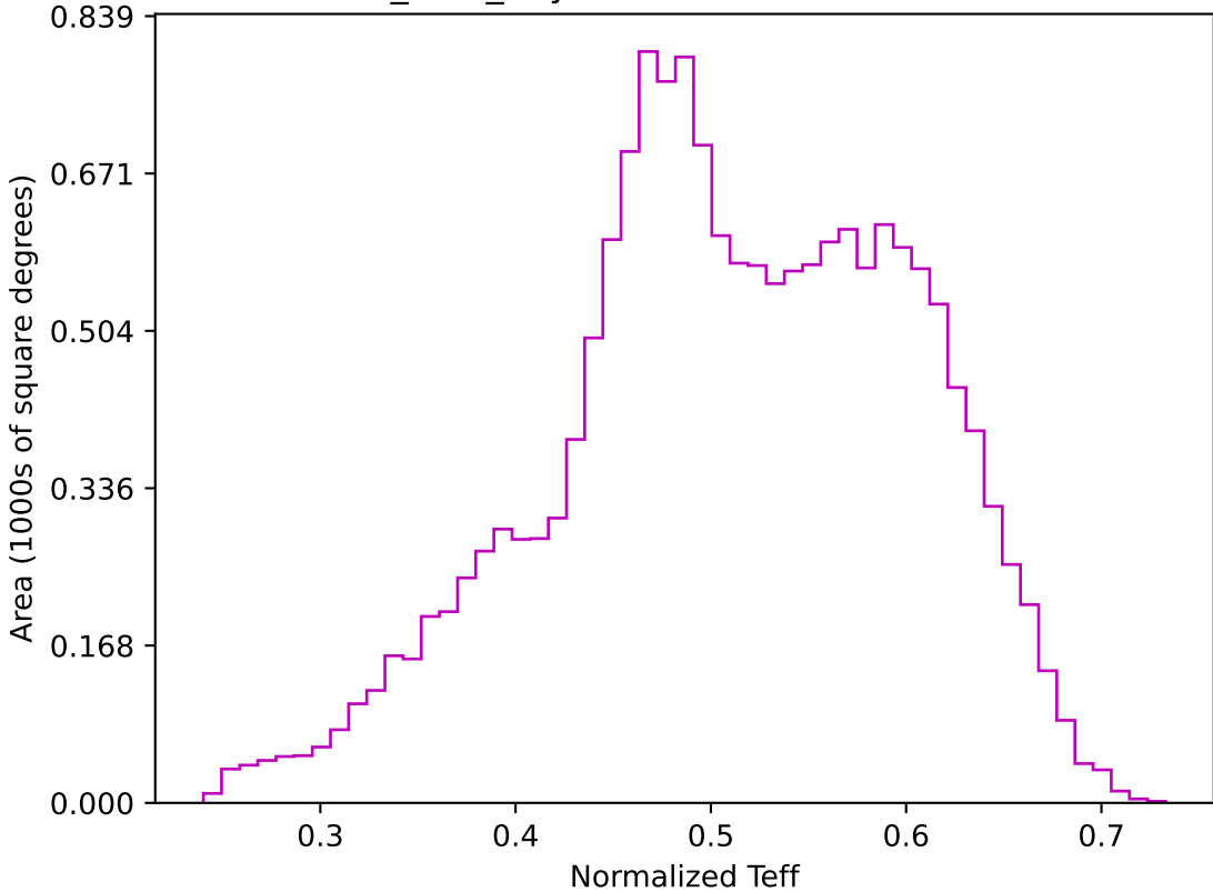
baseline_v3.0_10yrs WFD z band: Normalized Teff
