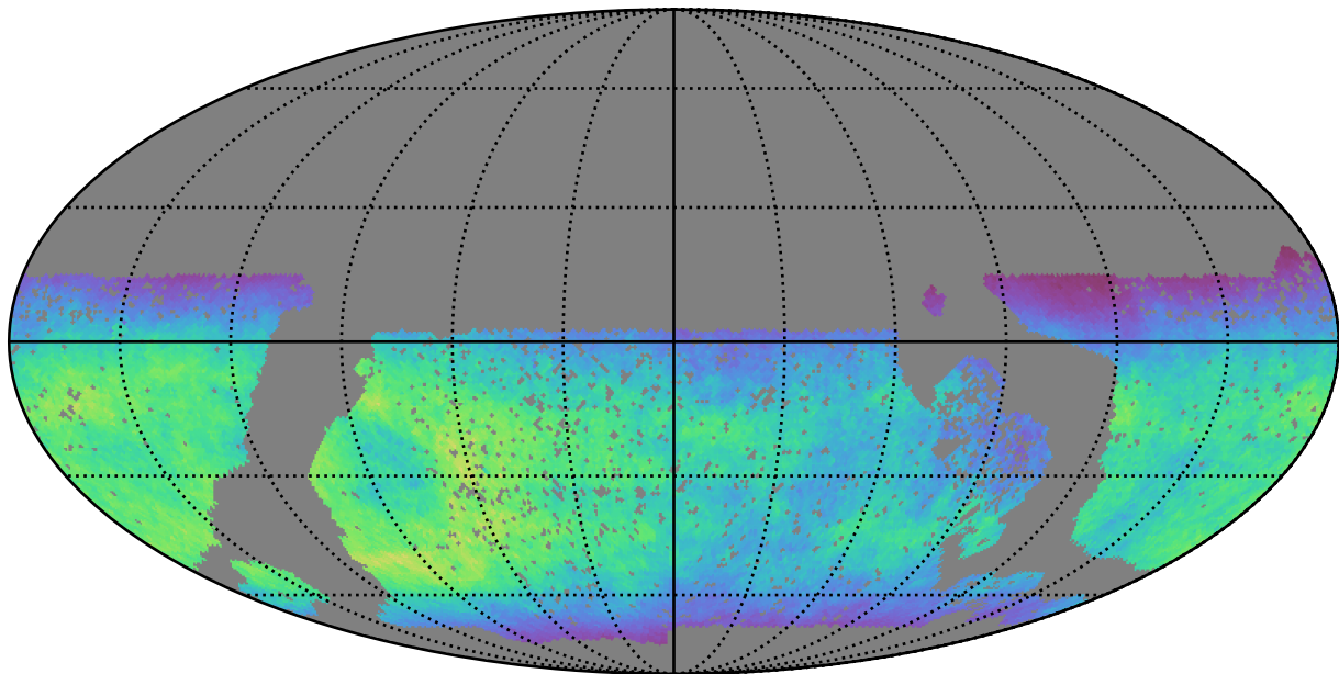
baseline_v3.0_10yrs WFD y band: Normalized Teff
