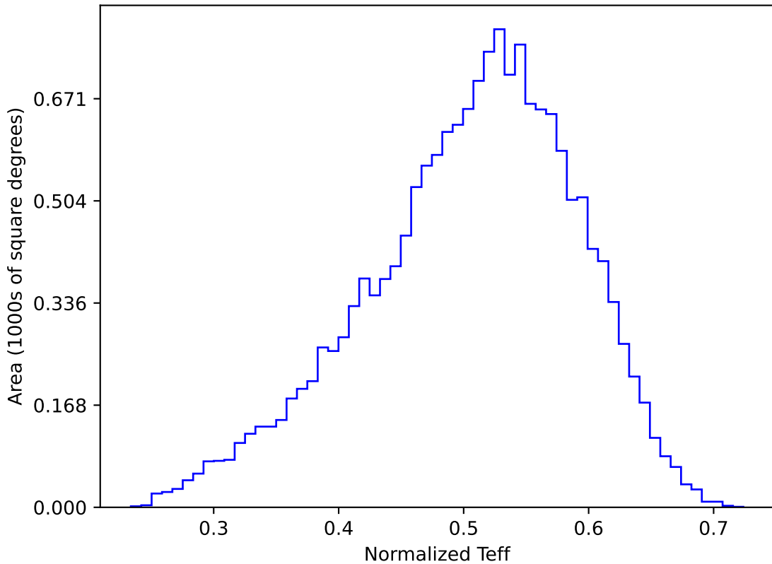
baseline_v3.0_10yrs WFD y band: Normalized Teff
