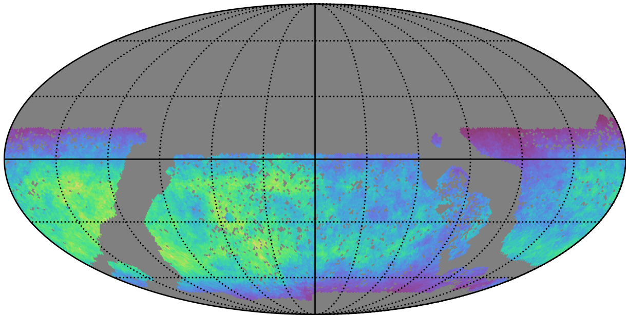
baseline_v3.0_10yrs WFD u band: Normalized Teff
