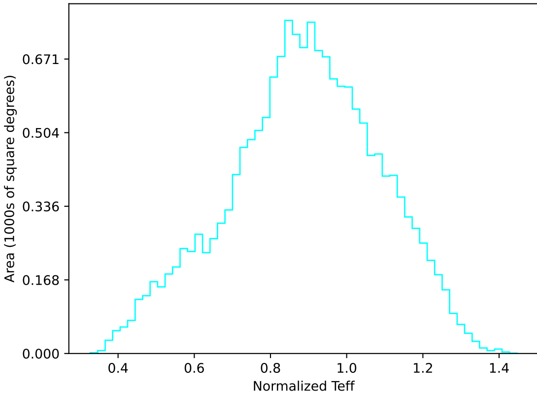
baseline_v3.0_10yrs WFD u band: Normalized Teff
