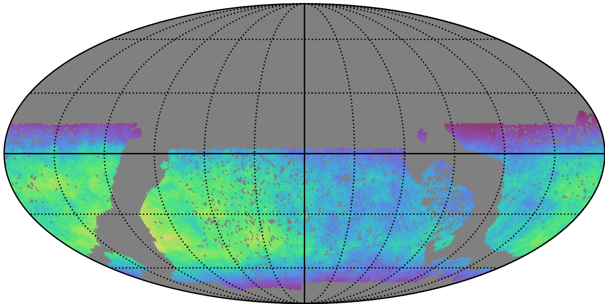
baseline_v3.0_10yrs WFD i band: Normalized Teff
