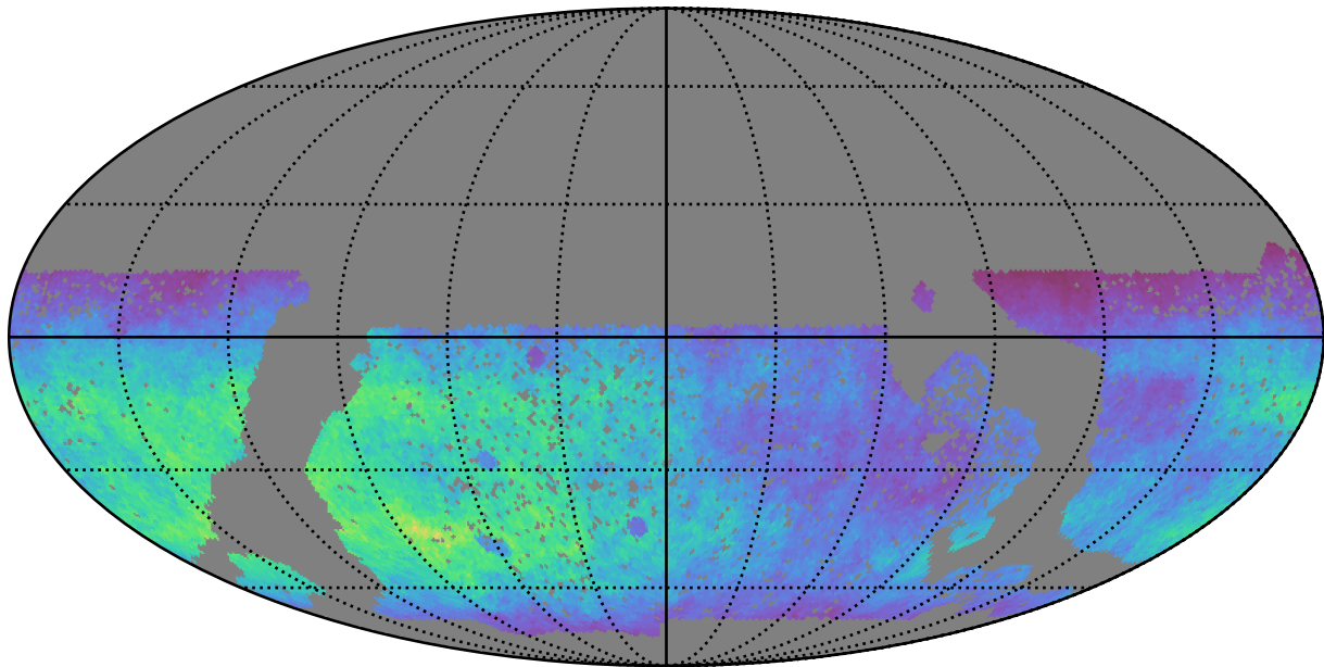
baseline_v3.0_10yrs WFD g band: Normalized Teff
