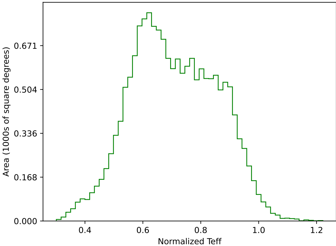
baseline_v3.0_10yrs WFD g band: Normalized Teff
