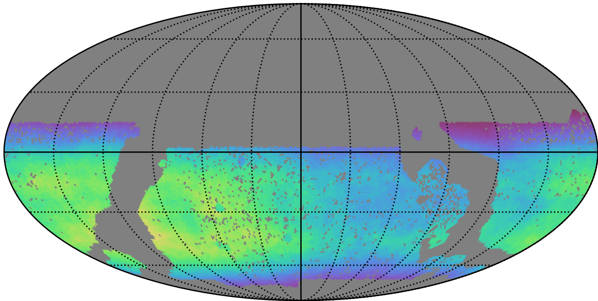
baseline_v3.0_10yrs WFD all bands: Normalized Teff
