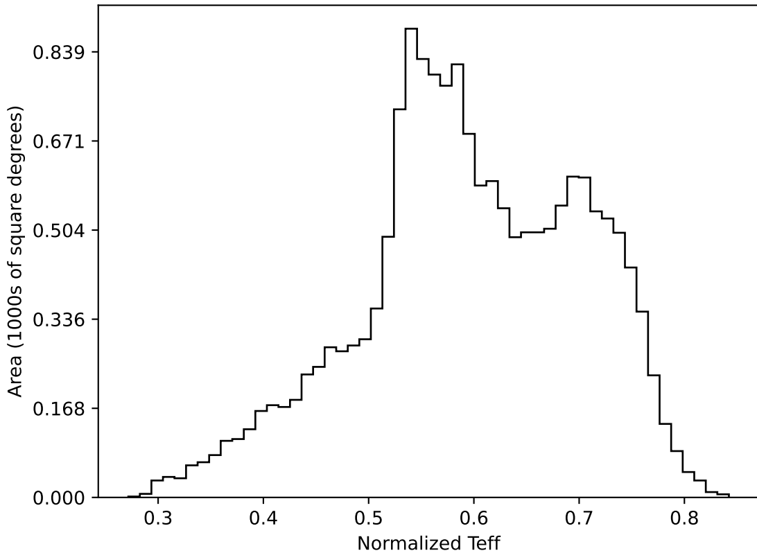
baseline_v3.0_10yrs WFD all bands: Normalized Teff
