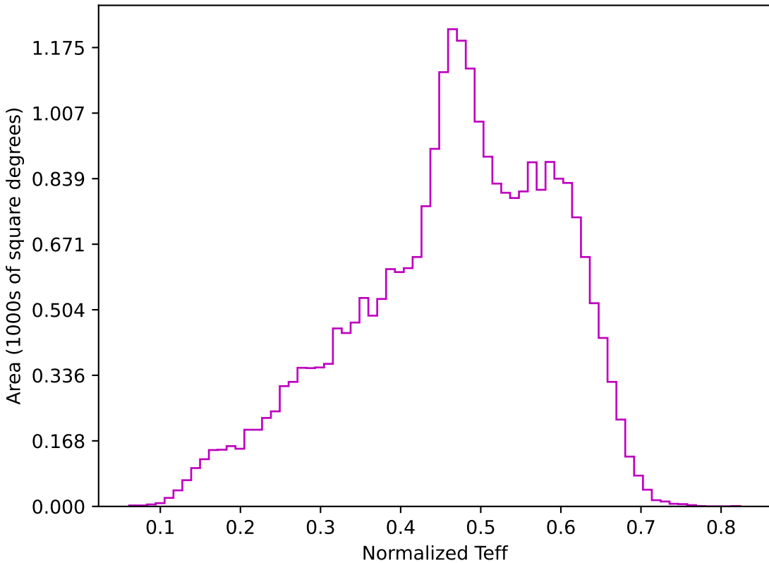
baseline_v3.0_10yrs All sky z band: Normalized Teff
