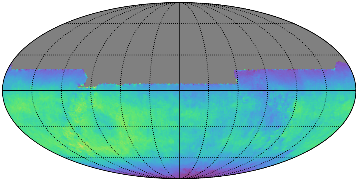
baseline_v3.0_10yrs All sky y band: Normalized Teff
