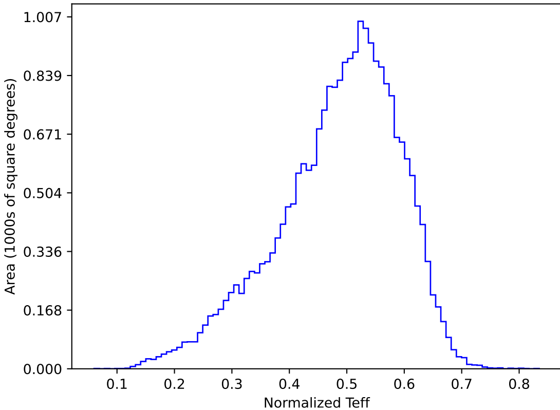
baseline_v3.0_10yrs All sky y band: Normalized Teff
