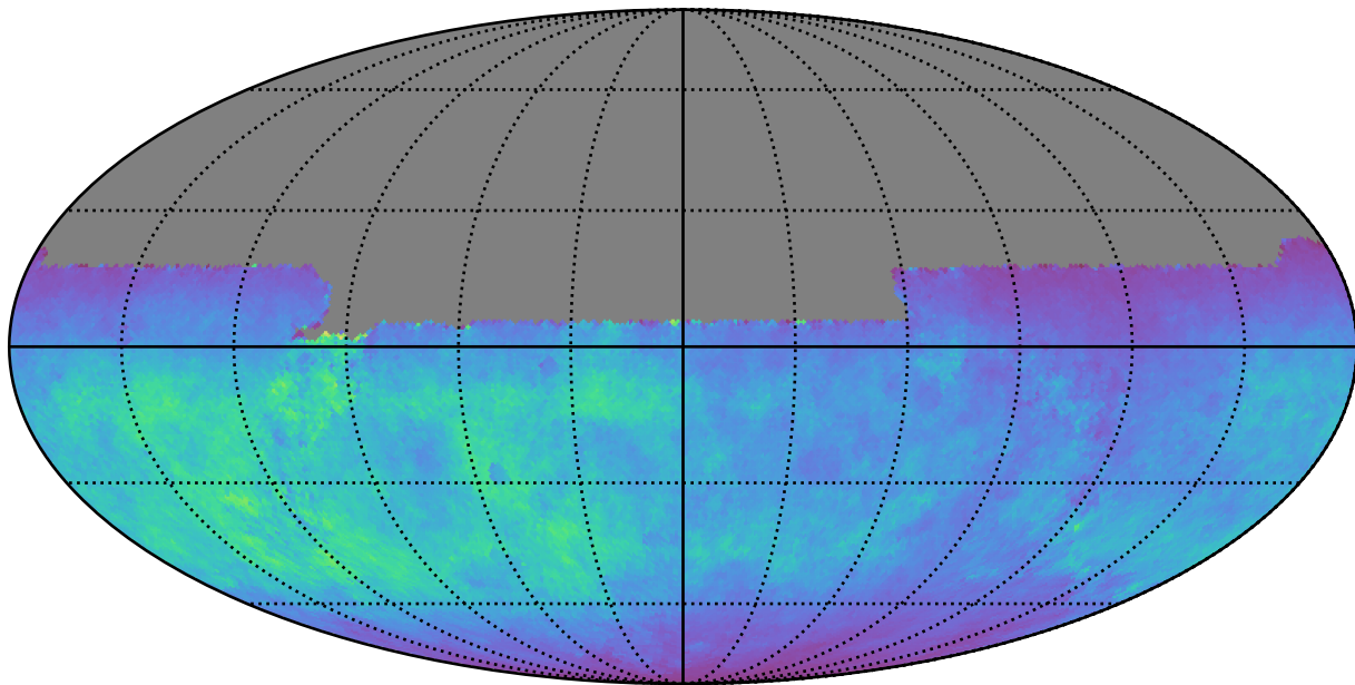
baseline_v3.0_10yrs All sky u band: Normalized Teff
