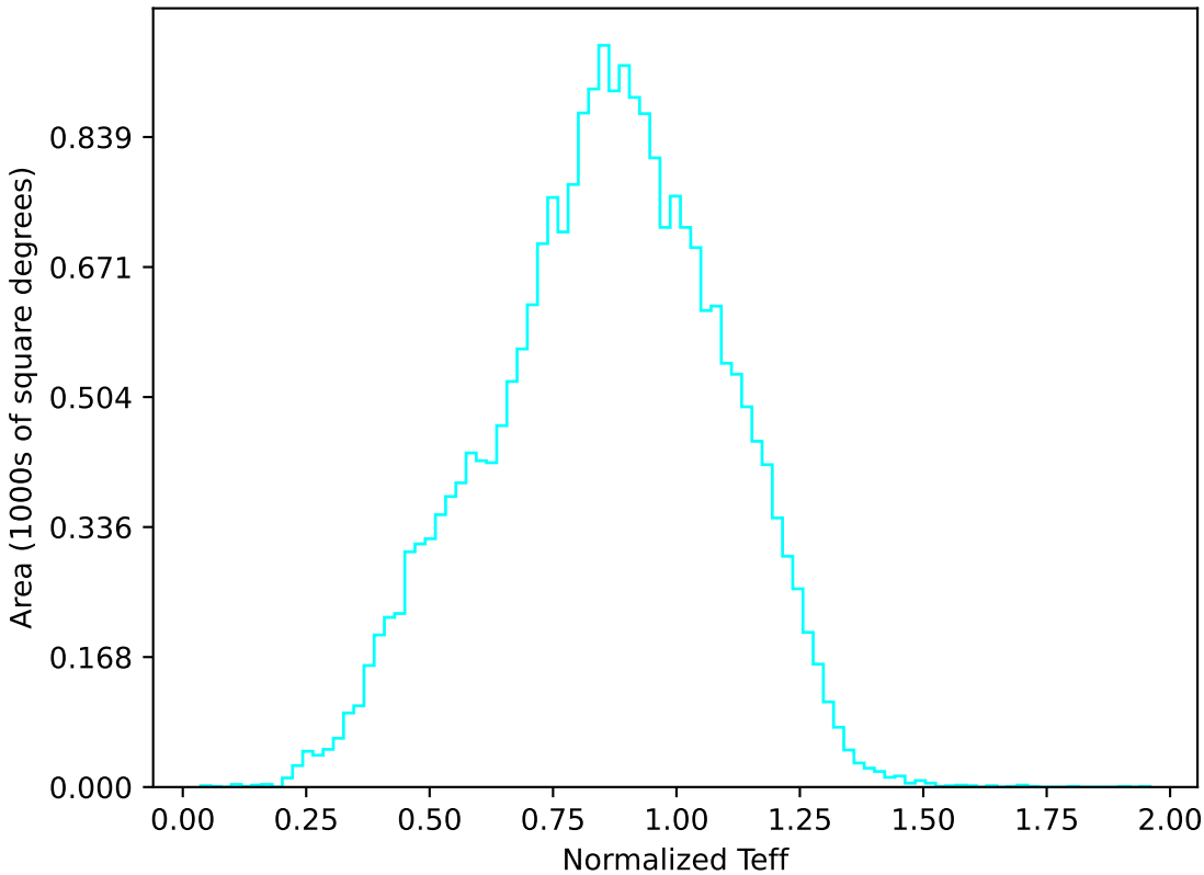
baseline_v3.0_10yrs All sky u band: Normalized Teff
