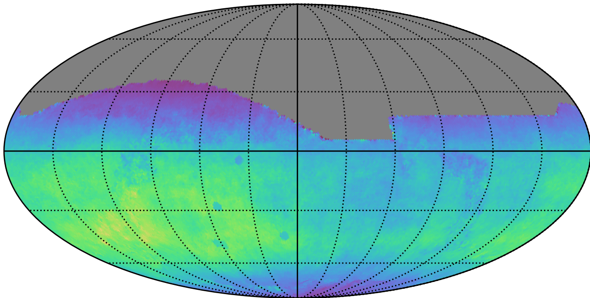
baseline_v3.0_10yrs All sky r band: Normalized Teff
