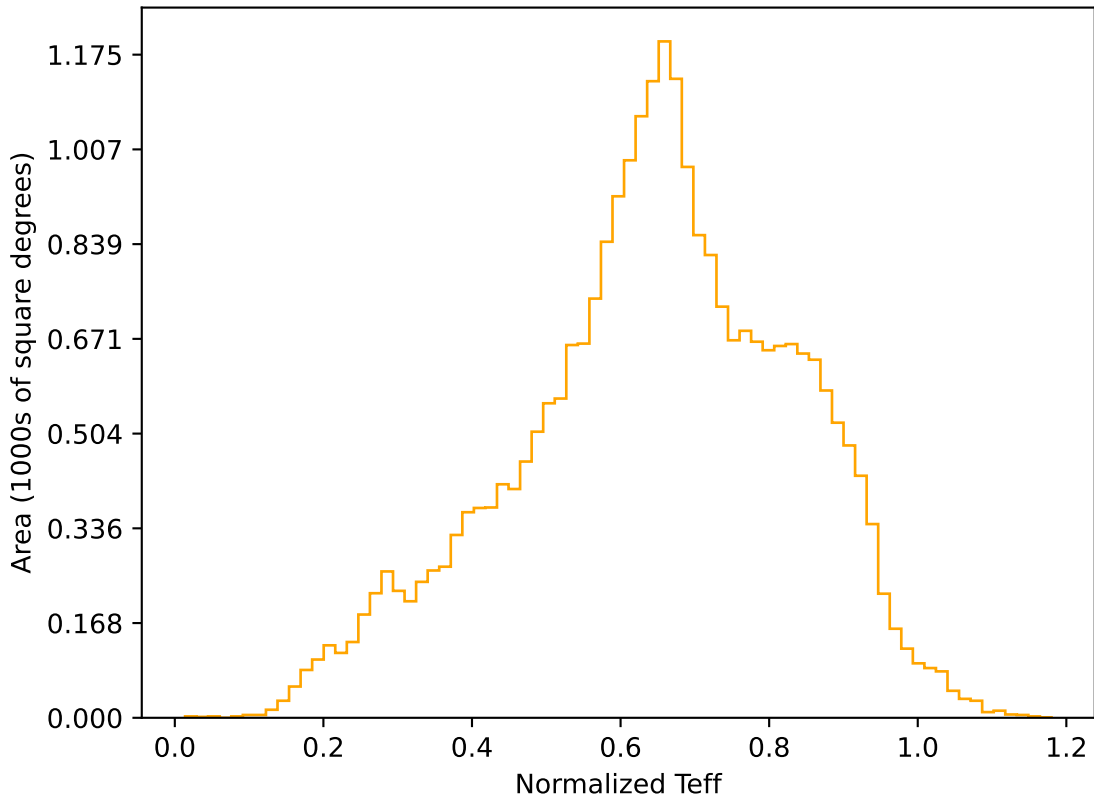
baseline_v3.0_10yrs All sky r band: Normalized Teff
