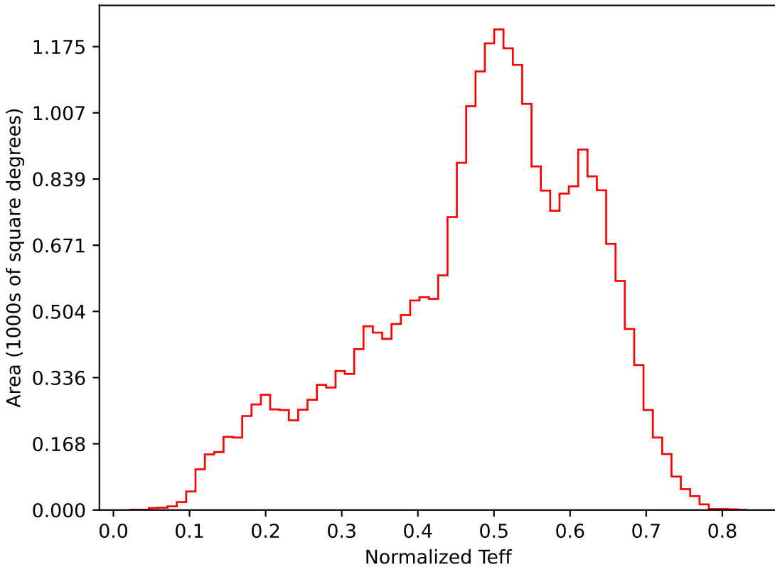
baseline_v3.0_10yrs All sky i band: Normalized Teff
